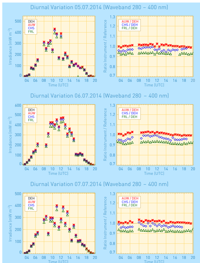
Figure 5: Diurnal variation of the global irradiance integrated over the wavelength interval of 280 to 400 nm. The absolute values are shown on the left hand side and the ratio between participants and reference instrument are shown on the right hand side.
