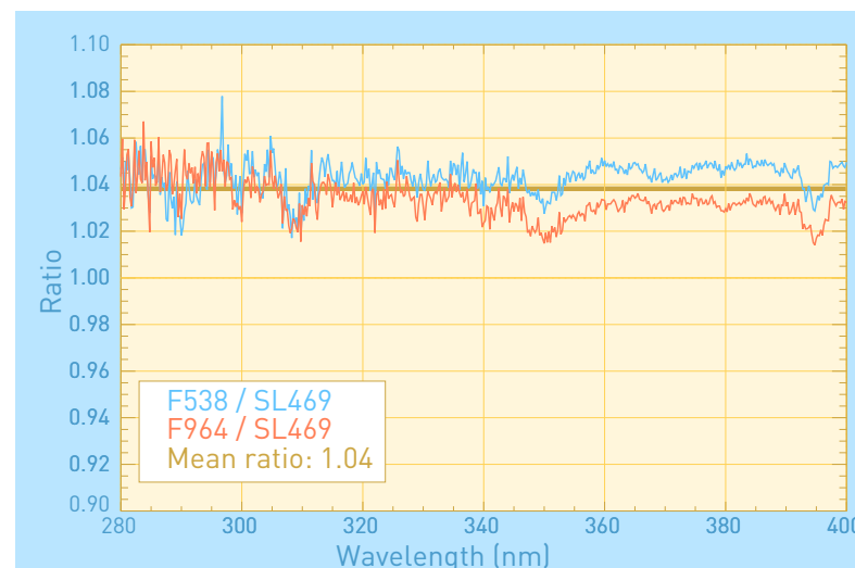
Figure 6: Ratio of FRL responsivity measurements performed with three different calibration lamps. The lamps with the identification number F538 and F964 are used by the French participants during their absolute calibration process. Lamp SL469 is used by the German group for their absolute calibration. A difference of about 4% between French and German calibration lamps is apparent.
