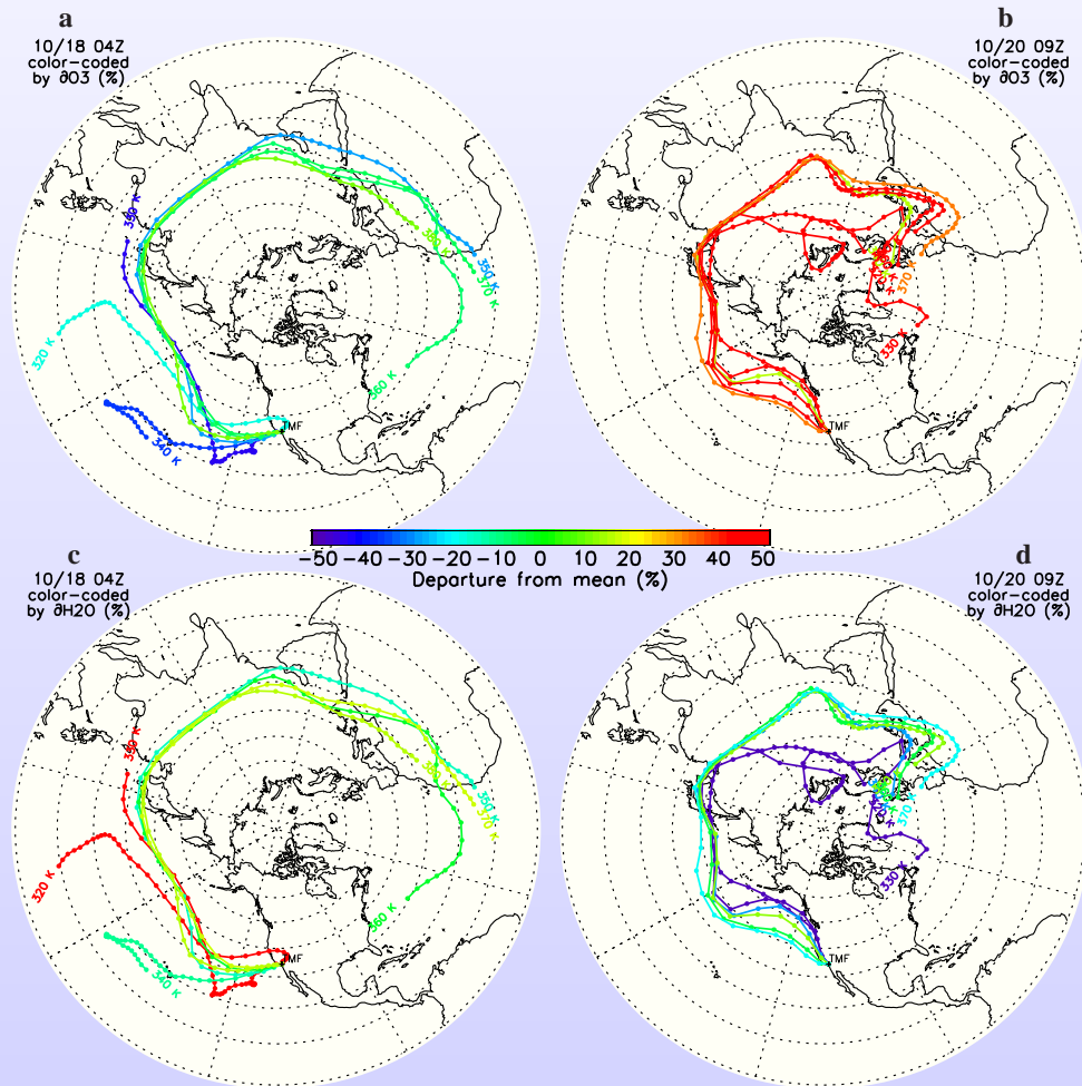
Figure 6: Selected 10-day back-trajectories ending over TMF on Oct. 18 (left) and 20 (right), 2009; top row: trajectories are colour coded by ozone anomalies with respect to the MOHAVE-2009 campaign mean; bottom row: trajectories are colour coded by water vapour anomalies.
