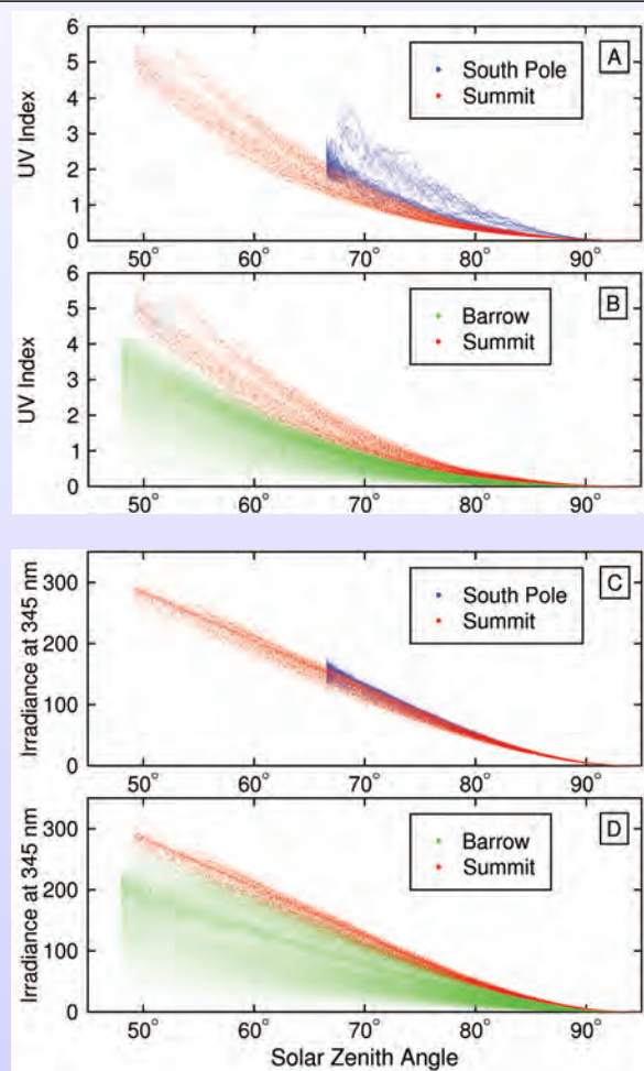
Figure 2: Comparison between sites and wavelengths of the SZA dependencies of measured irradiances. Upper panels (UV Index). Lower panels, UVA irradiance at 345 nm.
