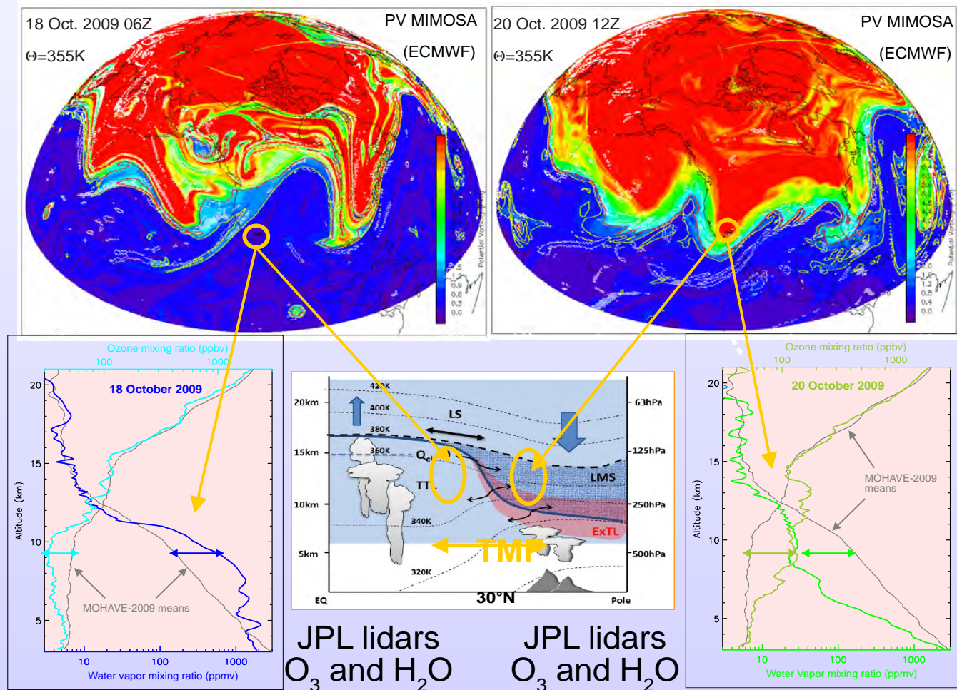
Figure 5: Schematic view, and demonstration by the observations, of what the JPL/TMF water vapour and ozone lidars sample when sounding layers located either north or south of the subtropical jet; top figures: Potential Vorticity maps produced by the high-resolution model MIMOSA.
