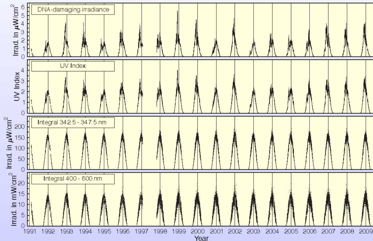
Figure 1: Irradiance time series at the South Pole.
