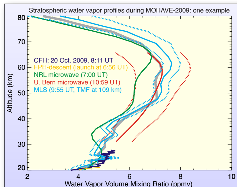
Figure 3: One example of simultaneous and co-located water vapour measurements, and their reported uncertainties, during MOHAVE-2009. The microwave measurements use 6-hour integration.
