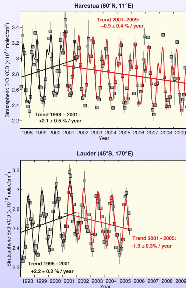
Figure 1: Trend analysis of stratospheric BrO columns over Harestua (60°N, 11°E; upper plot) and Lauder (45°S, 170°E; lower plot). More details in Hendrick et al. [2008].
