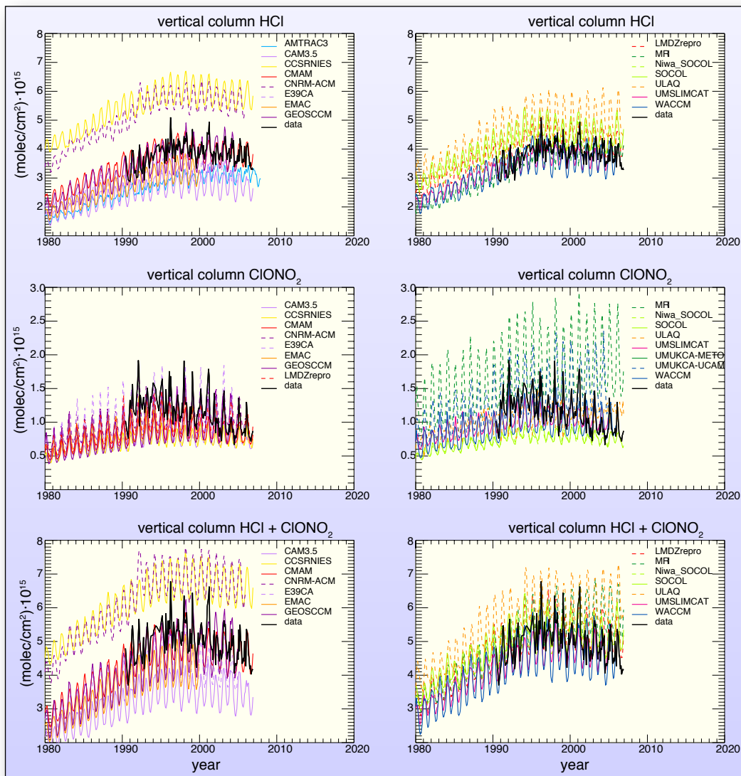
Figure 1. Comparison of NDACC observed column abundances (molecules·cm -2 ) of HCl, ClONO 2 , and their sum at Jungfraujoch (45°N) with output from 14 different CCMs from different groups. The models are divided arbitrarily between the left and right hand columns. Taken from SPARC CCMVal (2010) Chapter 6.
