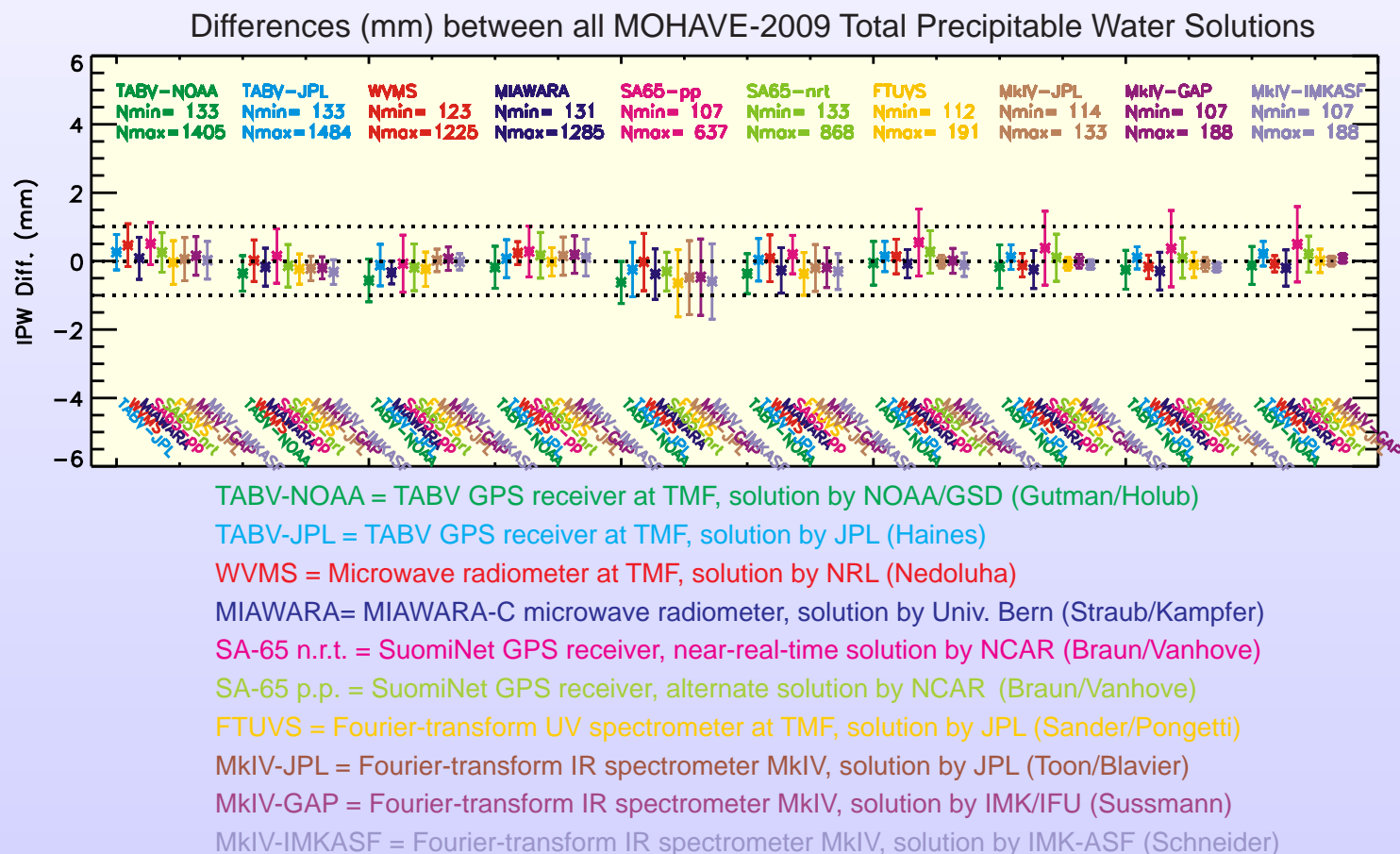
Figure 4: Comparison between all Total Precipitable Water Measurements made during MOHAVE-2009 (6 instruments, multiple retrievals for some instruments); Nmin and Nmax refer to the minimum and maximum number of pairs used for the comparisons; the vertical bars show the r.m.s. of the differences.
