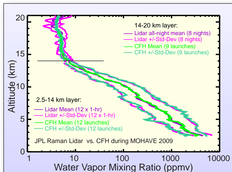
Figure 2: Campaign-mean and standard deviations of water vapour measured by lidar and CFH; a time coincidence and lidar integration time of 1 hour is used in the troposphere (below 14 km); a time coincidence of 6 hours and full-night lidar integration is used above 14 km.
