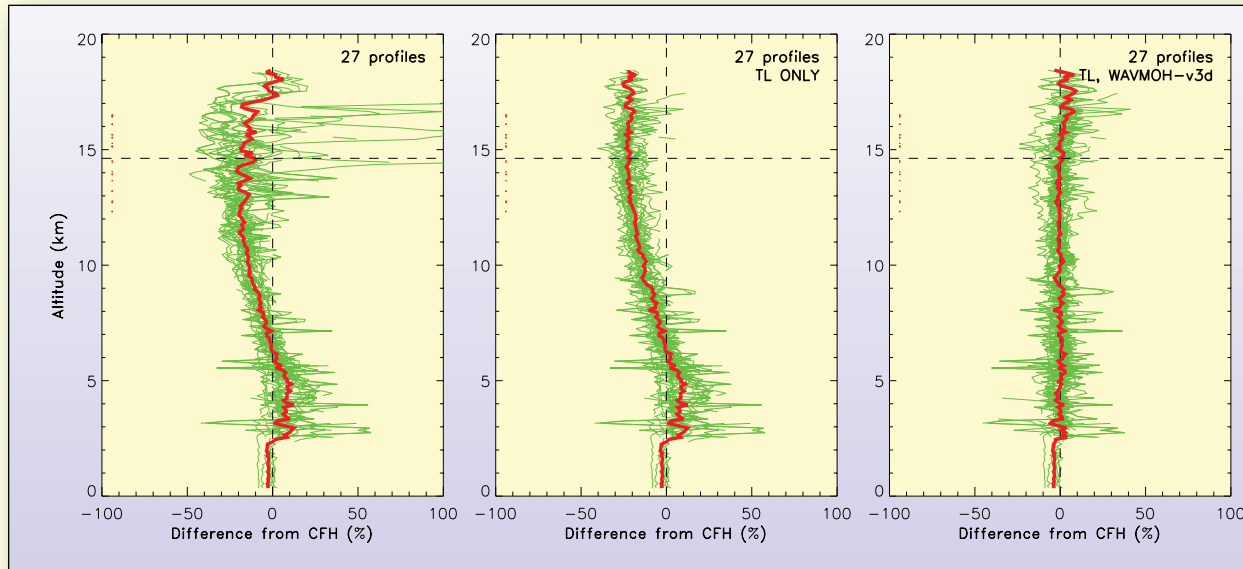
Figure 1. Left: percentage difference in relative humidity measurements of uncorrected Vaisala RS-92 and CFH. Middle: Same comparison after correction for the increasing response time of the Vaisala sensor with altitude. Right: Same comparison after application of the empirical correction to RS-92 data.
