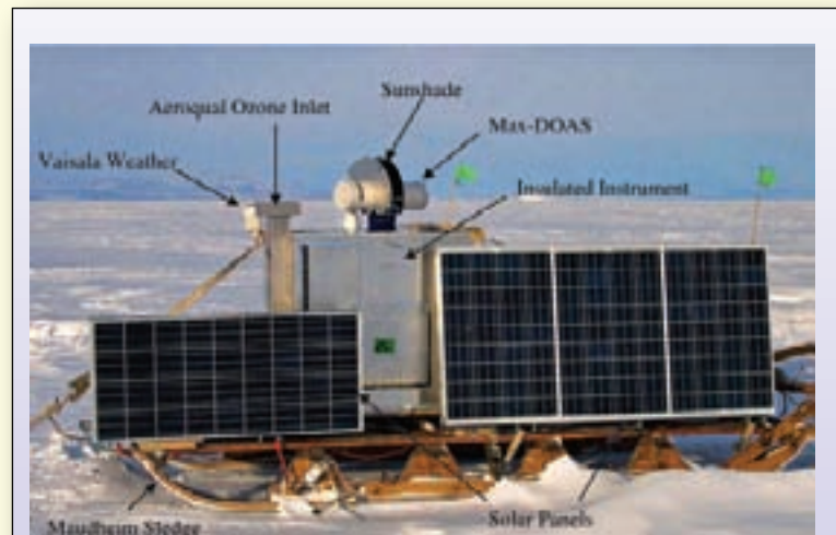
Photo 1. NIWA instrument platform and solar array on the Maudheim sledge on the sea ice.
