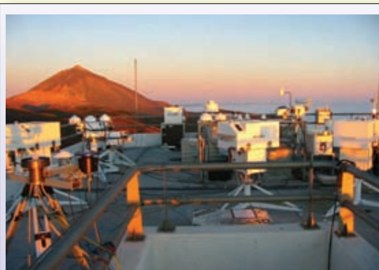
Photo 1. The double monochromator Brewer Spectrophotometer triad over the observation tower roof at the Izaña Observatory with other instruments.
