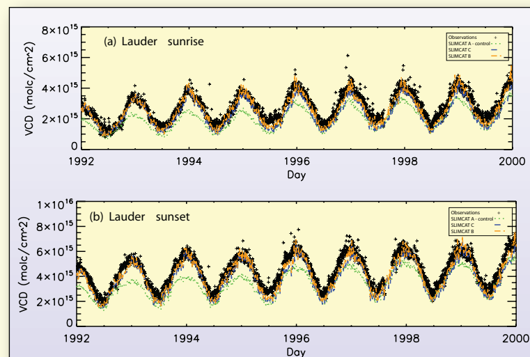
Figure 1. Observed vertical column of \text{NO}_2 (+ marks) at Lauder ( 45^\circ\text{S} , 170^\circ\text{E} ) at 90^\circ for (a) sunrise and (b) sunset from 1992 to 2000. Also shown are results from three SLIMCAT 3D model simulations: The basic model run A (green line), run B (orange line) with assimilation of HALOE \text{CH}_4 and \text{O}_3 , and run C (blue line) with assimilation of \text{CH}_4 only.
