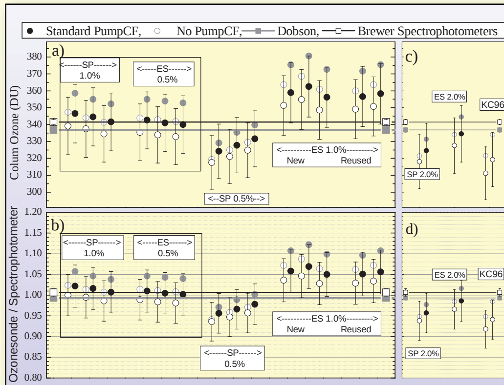
Figure 2. a) Integrated ozone from the 12 core ozonesondes (3 SP1.0, 3 ES0.5, 3 SP0.5, and 3 ES1.0), two reused ES1.0 ozonesondes, circles with error bars, and from Dobson and Brewer spectrophotometers located at the launch site, lines with boxes and error bars. The ozonesonde measurements are extrapolated using both the SBUV climatology (40 DU for April at 41°N) black circles filled and open [McPeters et al., 1997], and at constant ozone mixing ratio above the last ozone measurement, gray circles filled and open, without error bars. Results with and without the standard pump efficiency correction [Komhyr, 1986] for measurements at low air pressures are shown. The error bars indicate a precision of 5%. The standard deviation of the seven Dobson and Brewer spectrophotometer measurements completed during the balloon flight do not exceed the symbol sizes. b) As in a) but ratios of integrated total ozone from the ozonesondes to the average of the Dobson and Brewer measurements. c) and d) Same as a) and b) for the other 4 auxiliary ozonesondes flown (1 SP2.0, 1 ES2.0, 2 KC96). Results from the manufacturer's recommendations for solution strength are enclosed in the box in a) and b).
