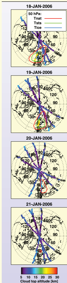
Figure 2. Cloud top height measured by MIPAS on 18-21 January 2006. Isotherms for the formation of NAT, STS and ice are shown in red, green and blue, respectively.
